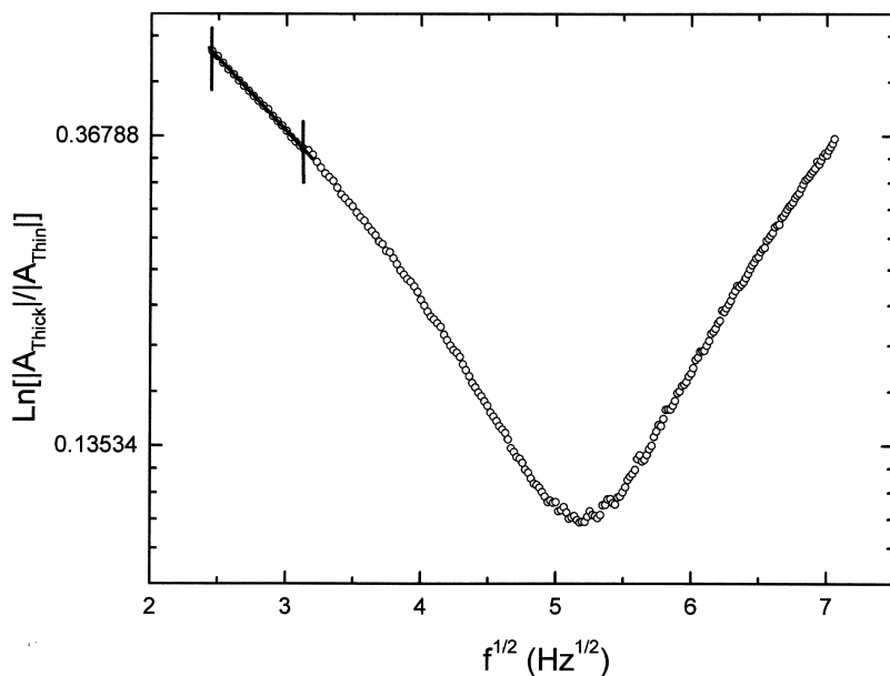
FIGURE 3 Photoacoustic signal amplitudes ratio for the Degufill (auto) resins samples of Figure 2. The linear behavior in the thermally thick regime is delimited by two vertical lines. The continuous straight line is the best fit to Eq. (3) within this region.
