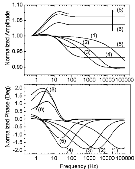
FIG. 7. Same as in Fig. 3 with coating thickness=500 \mu\text{m} ; k_c=38.80 W/m K and \alpha_c=10.74 \times 10^{-6} m 2 /s.
