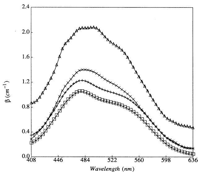
FIG. 6. Optical absorption spectra of \text{Ti}^{3+}:\text{Al}_2\text{O}_3 crystals, obtained with PPES in the purely optical transmission mode, Eq. (15), at f = 9 \text{ Hz} . ( \triangle - \triangle - \triangle ): l = 0.0813 \text{ cm} , FOM = 40; ( \times - \times - \times ): l = 0.1295 \text{ cm} , FOM = 800; (+-+-+): l = 2.0169 \text{ cm} , FOM = 40; and ( \square - \square - \square ): l = 2.0125 \text{ cm} , FOM = 800.
