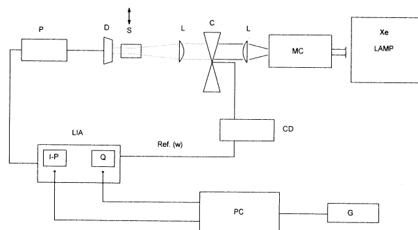
FIG. 5. Schematic of noncontact PPES spectrometer. MC, monochromator; L , lens; C , chopper; S , sample; D , detector; P , preamplifier with adjustable band-pass filters; LIA, lock-in amplifier (EG&G Model 5209 in the IP and Q modes); CD, chopperdriver; PC, computer for data acquisition, processing, and theoretical analysis; G , graphics and plotter.
